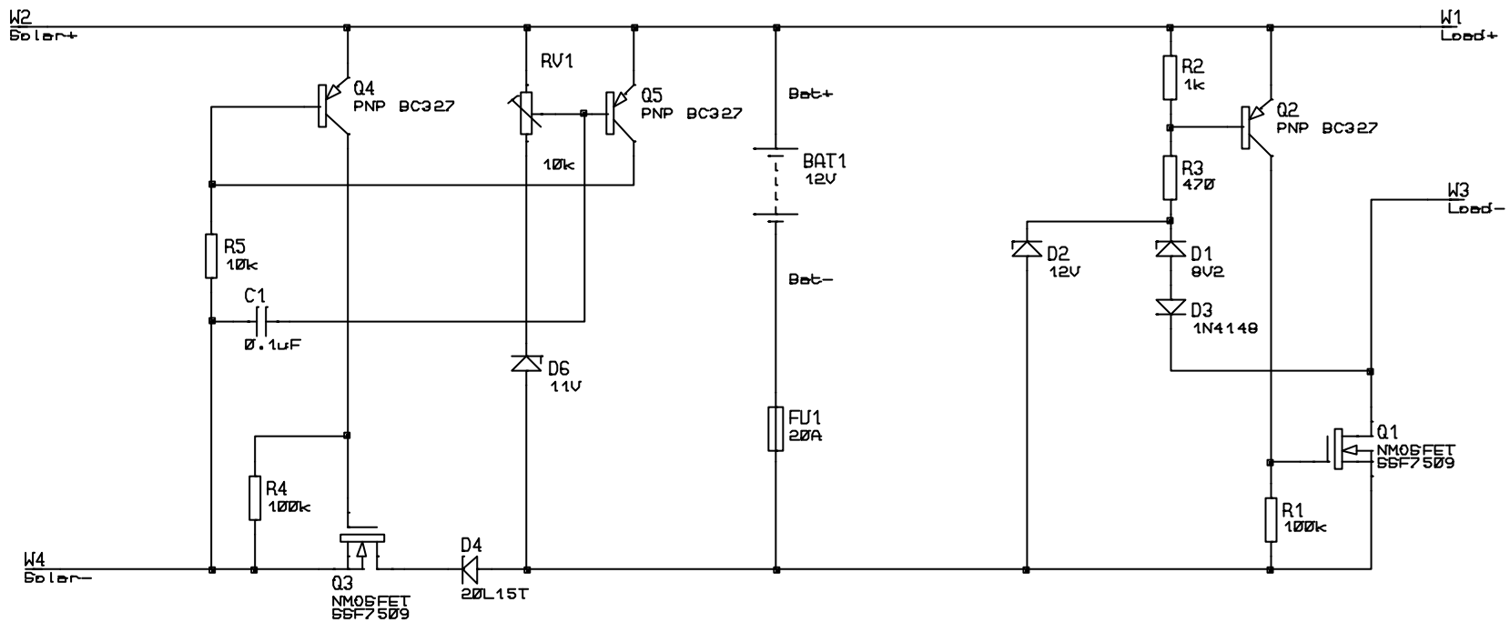
Load Switch
